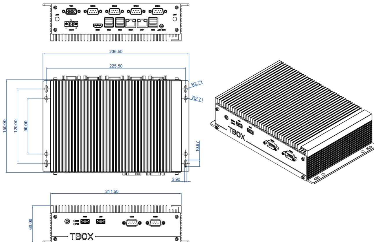
DIMENSIONAL DRAWING:TBOX-28X0
