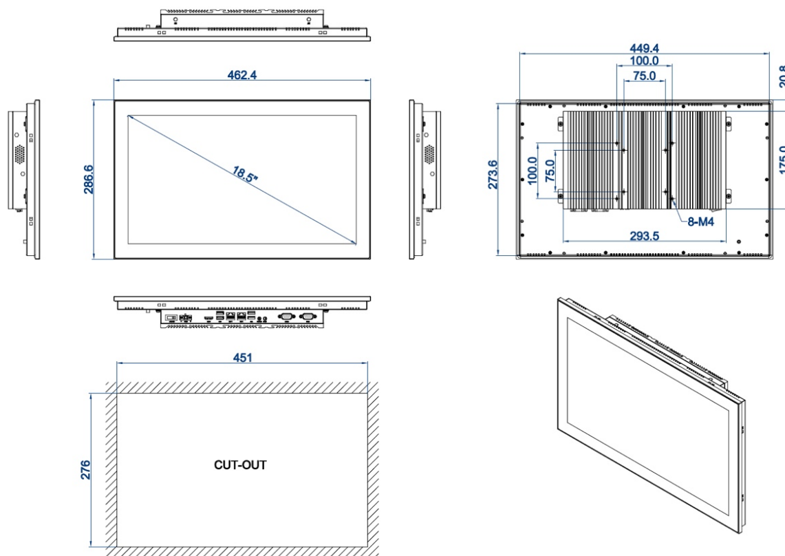
DIMENSIONAL DRAWING:TPC-DCM185
