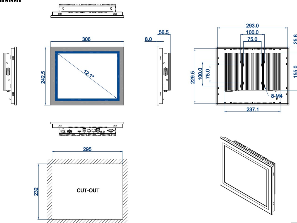
DIMENSIONAL DRAWING:TPC-DRM121
