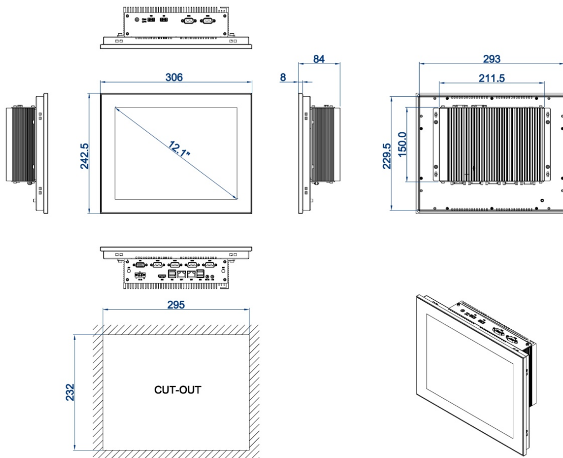
DIMENSIONAL DRAWING:TPC-PC121
