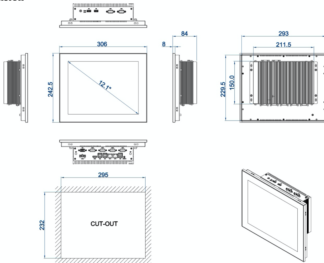
DIMENSIONAL DRAWING:TPC-PC121W
