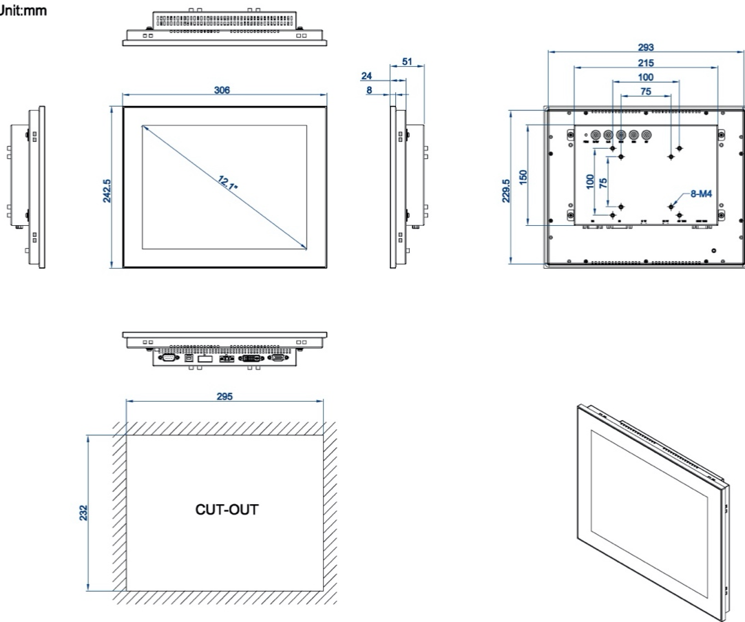
DIMENSIONAL DRAWING:TM-PC121
