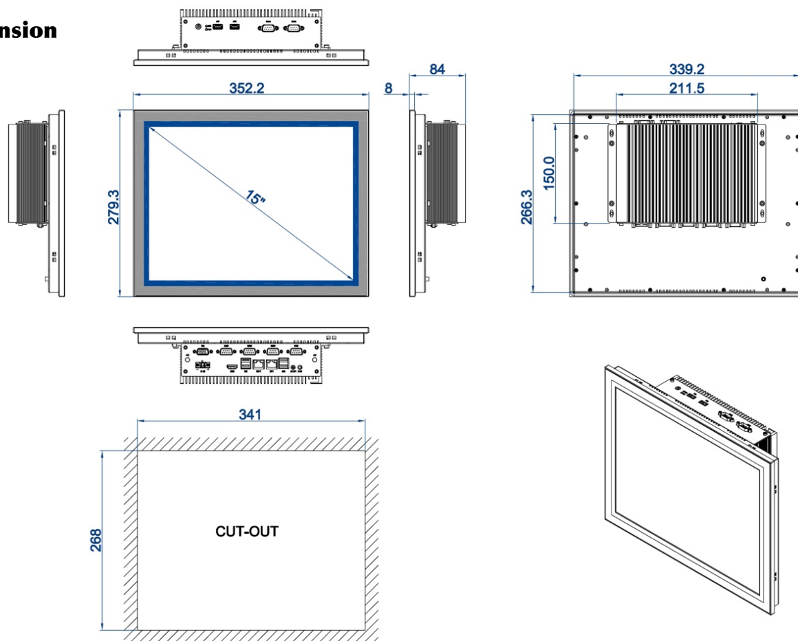
DIMENSIONAL DRAWING:TPC-PR150
