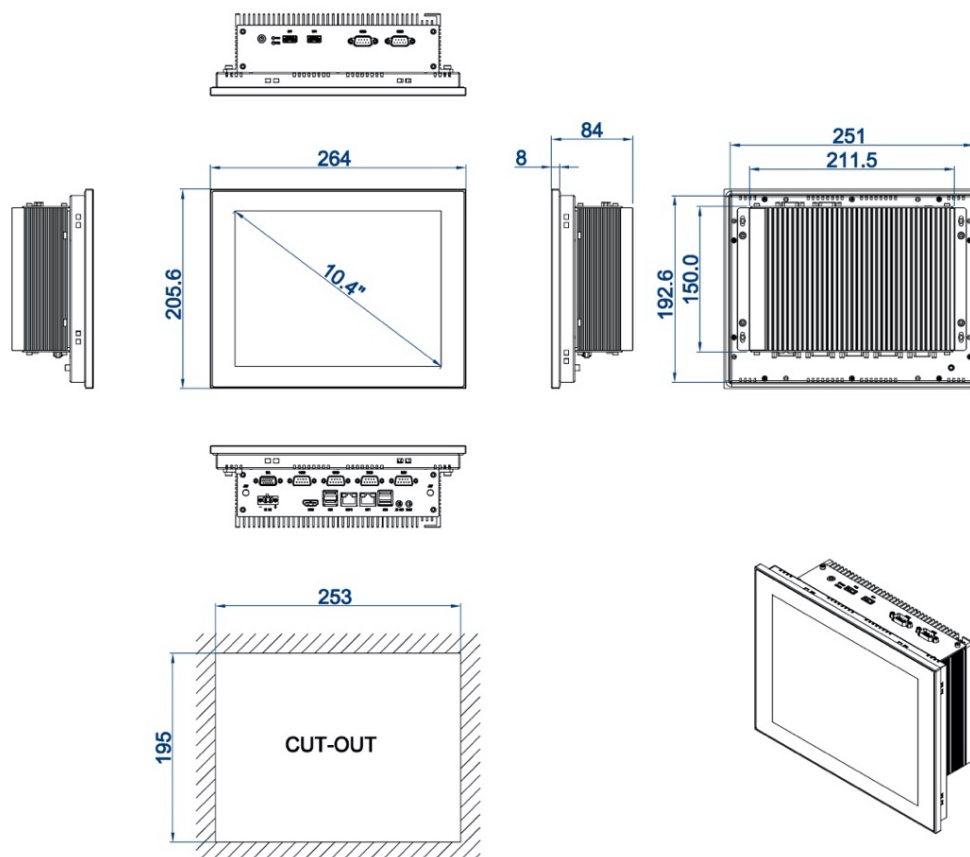
DIMENSIONAL DRAWING:TPC-PC104
