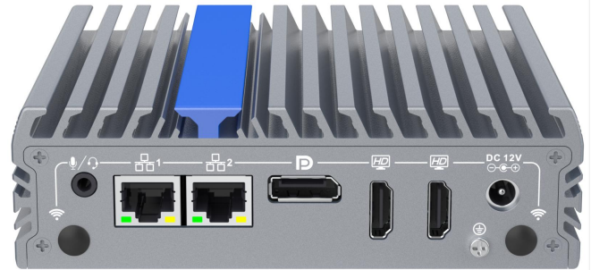
WIFI AUDIO LANx2 DP HDMIx2 DC12V WIFI
